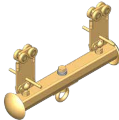
.T103 (2 x.T47 trolley)
