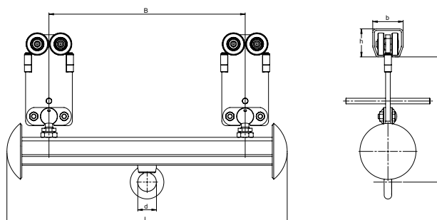
.T101 (2 x.T47 trolley)
