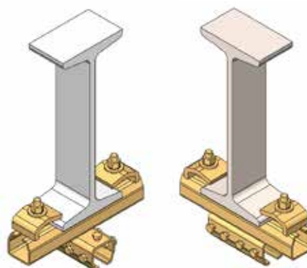
.B71 Parallel to the I-beam
