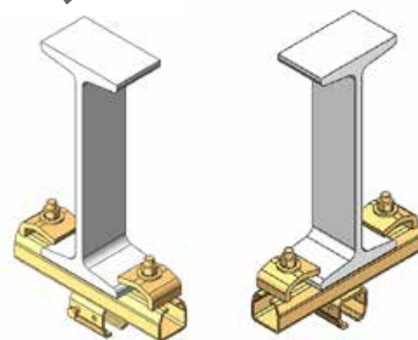
.B36 90° to the I-beam
