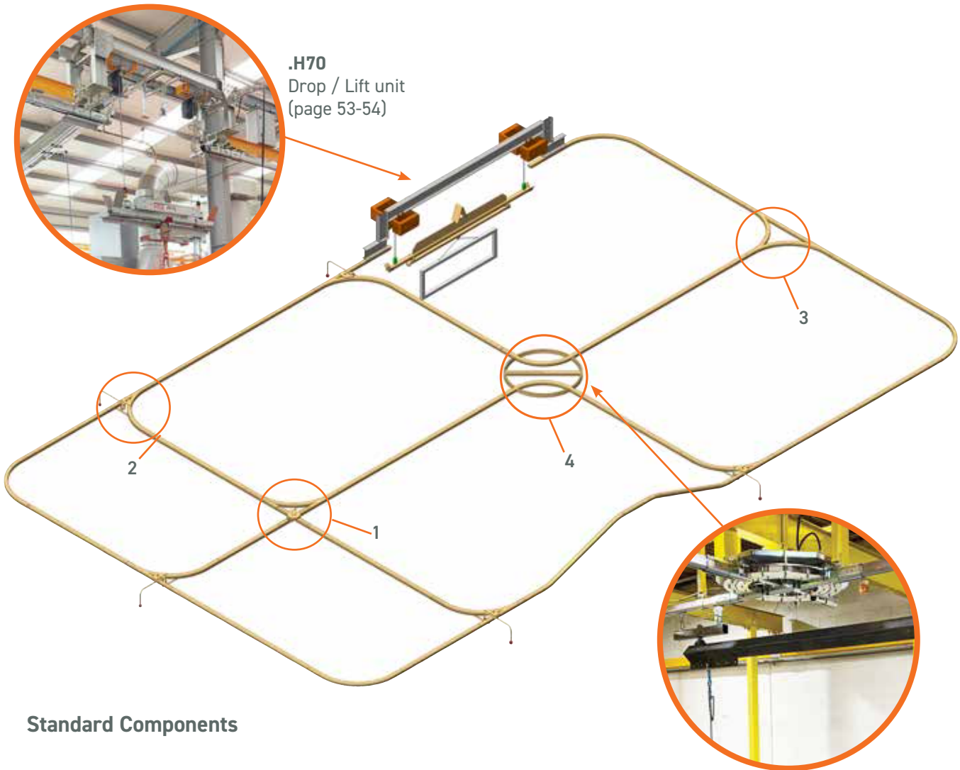
1 .A17 Tongue Switch with Pneumatic turn table (page 40)
