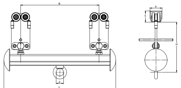
.T101 (2 x.T47 trolley)
