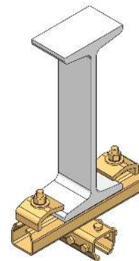
Parallel to the I-beam
